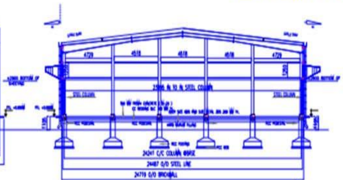
SECTIONAL ELEVATION
